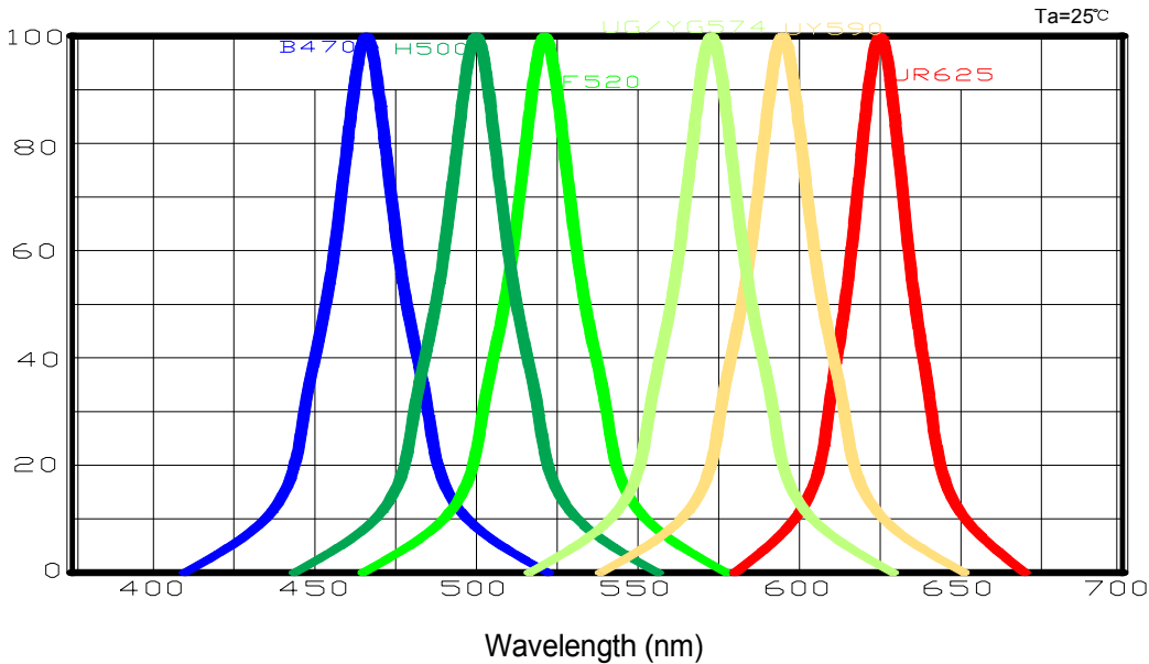
Wavelength Characteristics
